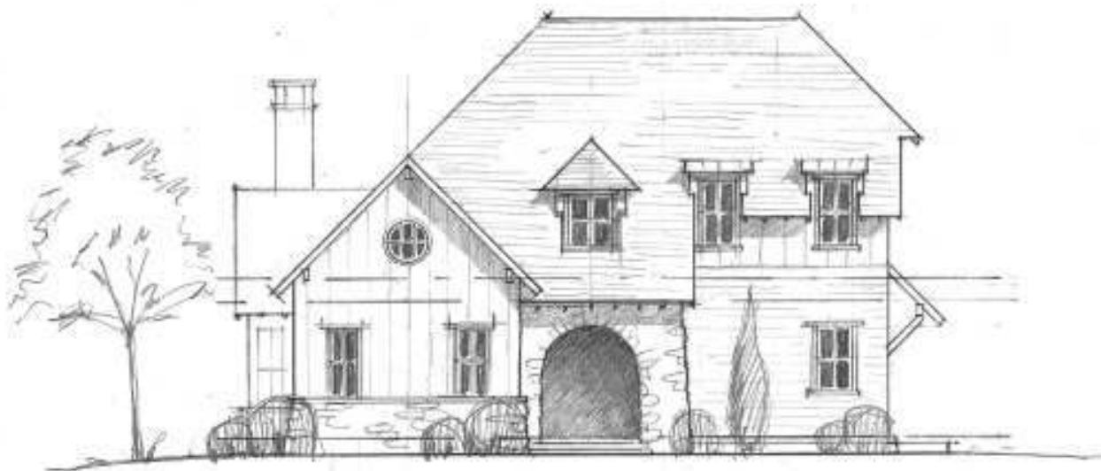
① SETTLEMENT COTTAGE (OPTION #2) FRONT ELEVATION SCALE: 1/8" = 1'-0"
